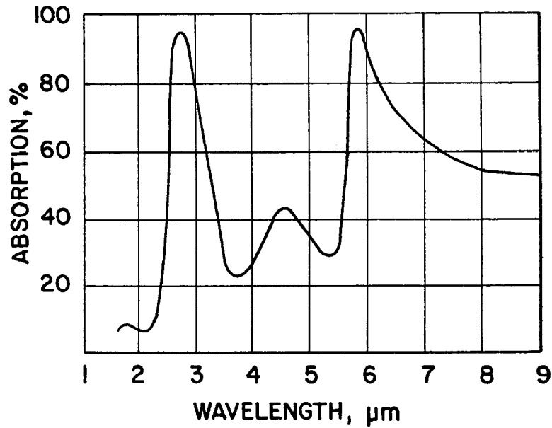
SPECTRAL ABSORPTION CURVE FOR WATER
